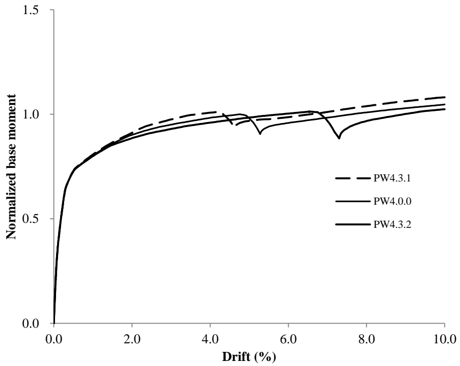
Figure 6.7(d): Parametric wall 4 with constant initial PT force
