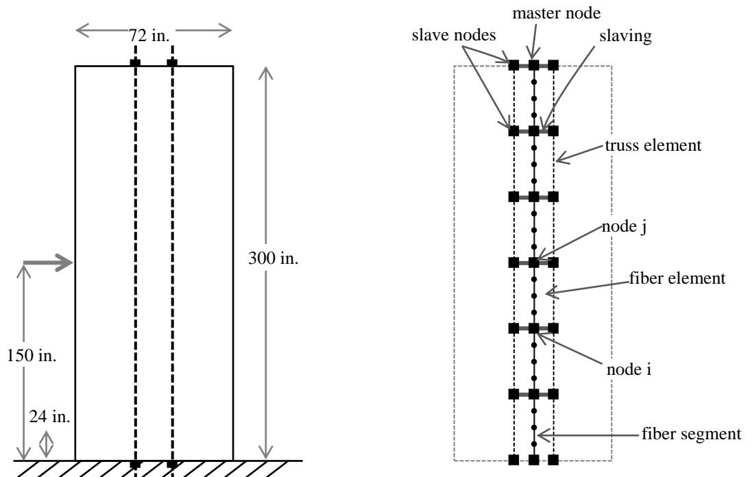
(a) Reinforcement detailing of PW1.0.0
