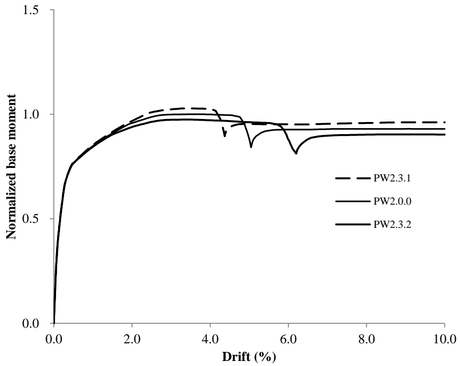
Figure 6.7(b): Parametric wall 2 with constant initial PT force
