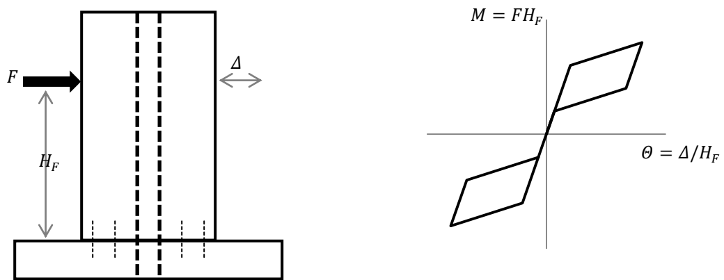
(c) Unbonded post-tensioned hybrid precast concrete wall and base moment-lateral drift curve
