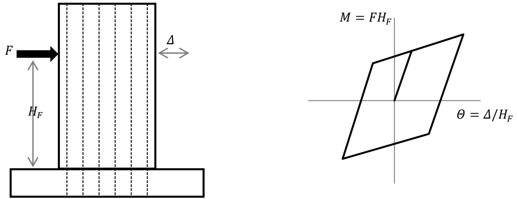
(a) ACI compliant cast-in-place wall and base moment-lateral drift curve
