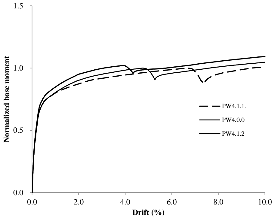
Figure 6.5(d): Parametric wall 4 with varying area of PT steel
