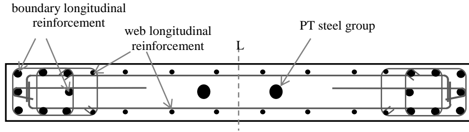
(a) Wall section with longitudinal reinforcement
