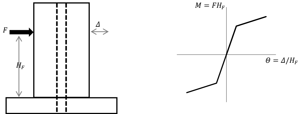
(b) Unbonded post-tensioned precast concrete wall and base moment-lateral drift curve
